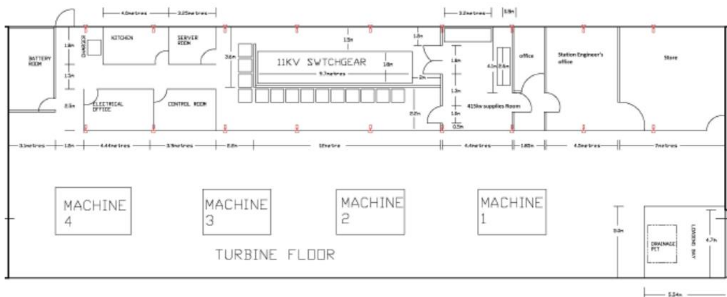
Schematic 1: Wanjii powerhouse floor plan
